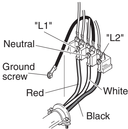
3-wire Cord Installed
