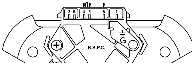
SWITCH SHOWN IN START POSITION
