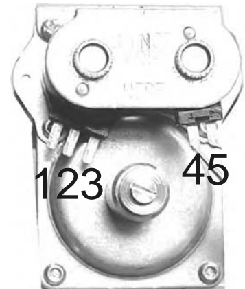
Gas Valve
