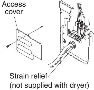
3-wire Cord Installed
