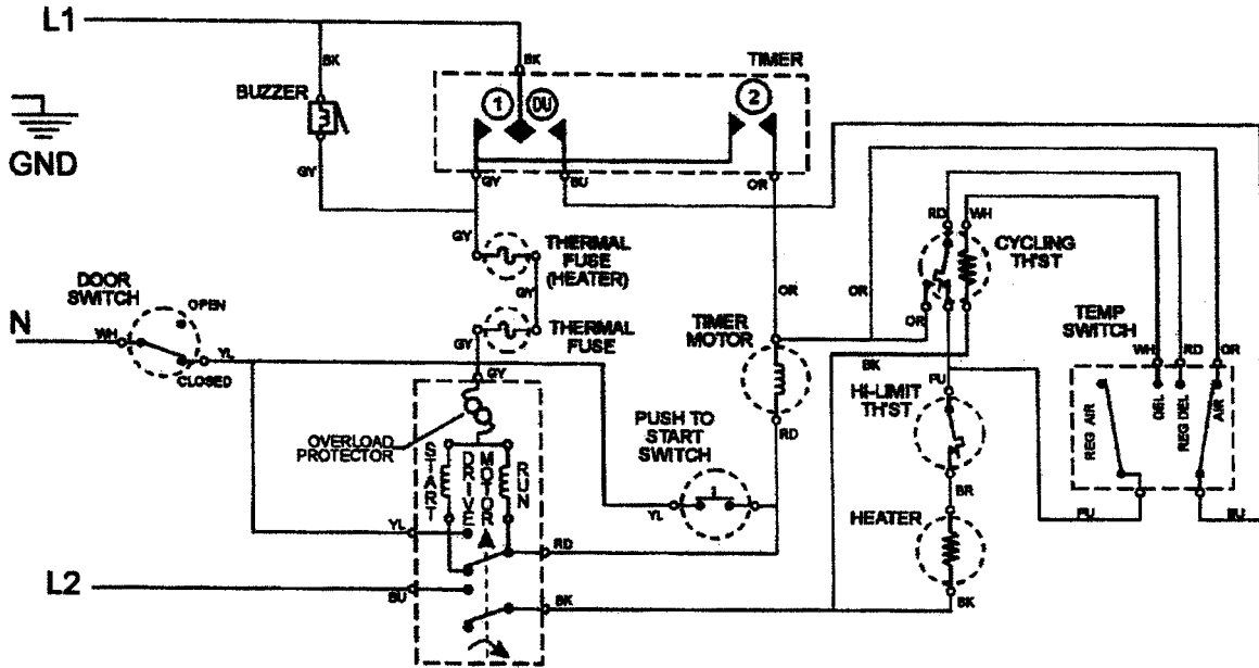
ELECTRICAL SCHEMATIC
