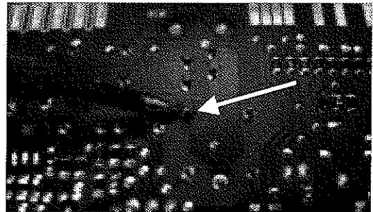
Burned board -- showing burned terminal on back of pc board.
