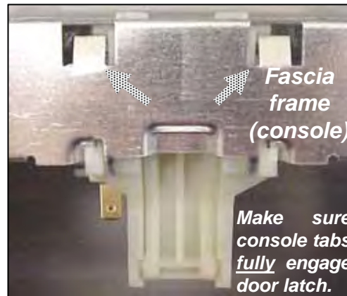
Bend tabs down into latch
