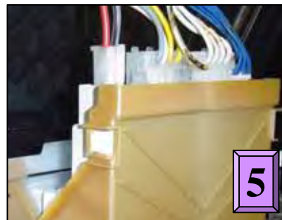
Removing wire harnesses
