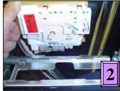
Snapping module into console
