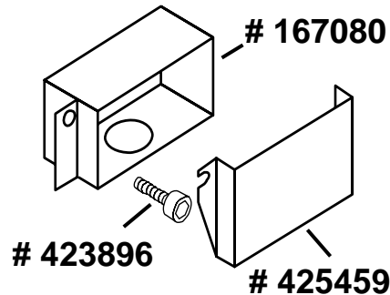
Old terminal box with cover
