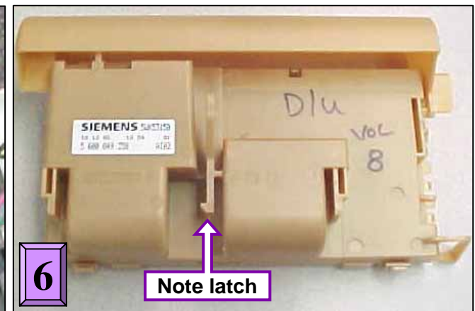
6 Aligning module tabs when reassembling
