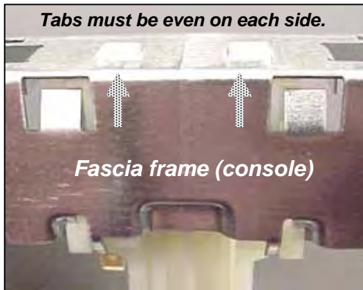
Insert latch tabs into frame
