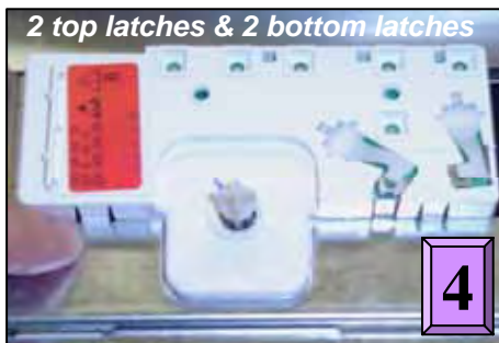
Unlatching module from console
