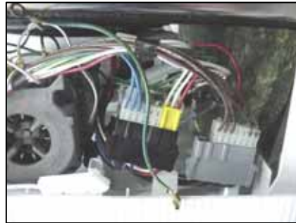
Removing terminal blocks from base
