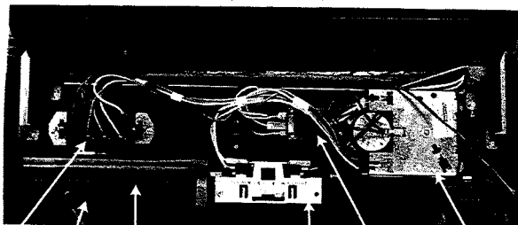
CONTROL SWITCH VENT LINER AREA DOOR LATCH SWITCH ASSEMBLY CYCLE EXTENDER TIMER
