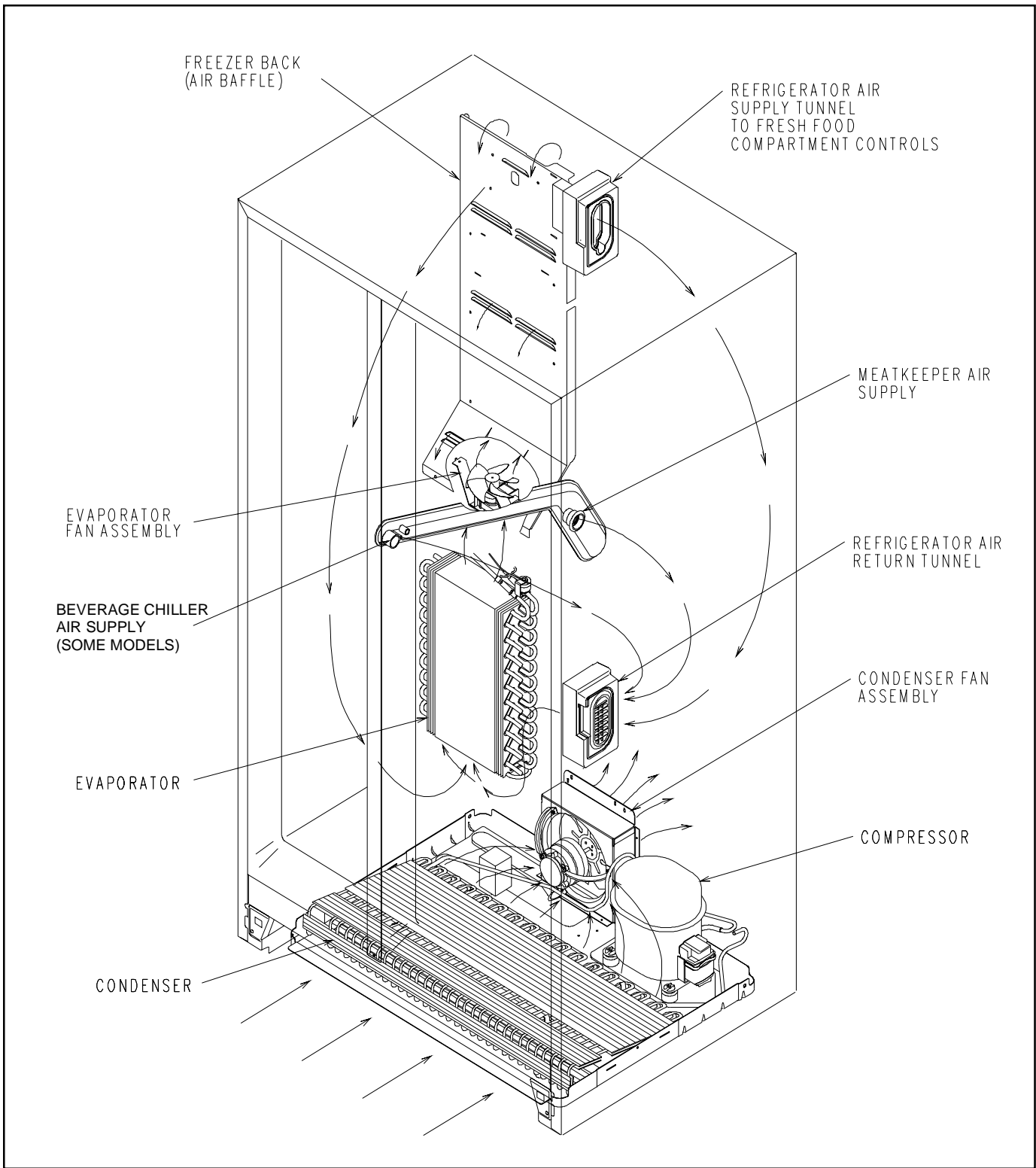
"T" Model Side x Side Air Flow Diagram 22/25/27 Cubic Foot Only
