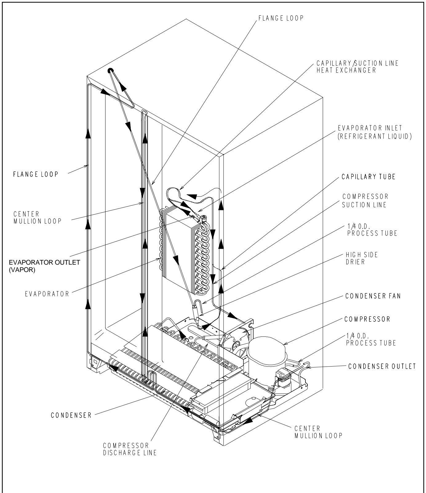
“T” Model Side x Side Refrigerant Flow Diagram 20 Cubic Foot Only
