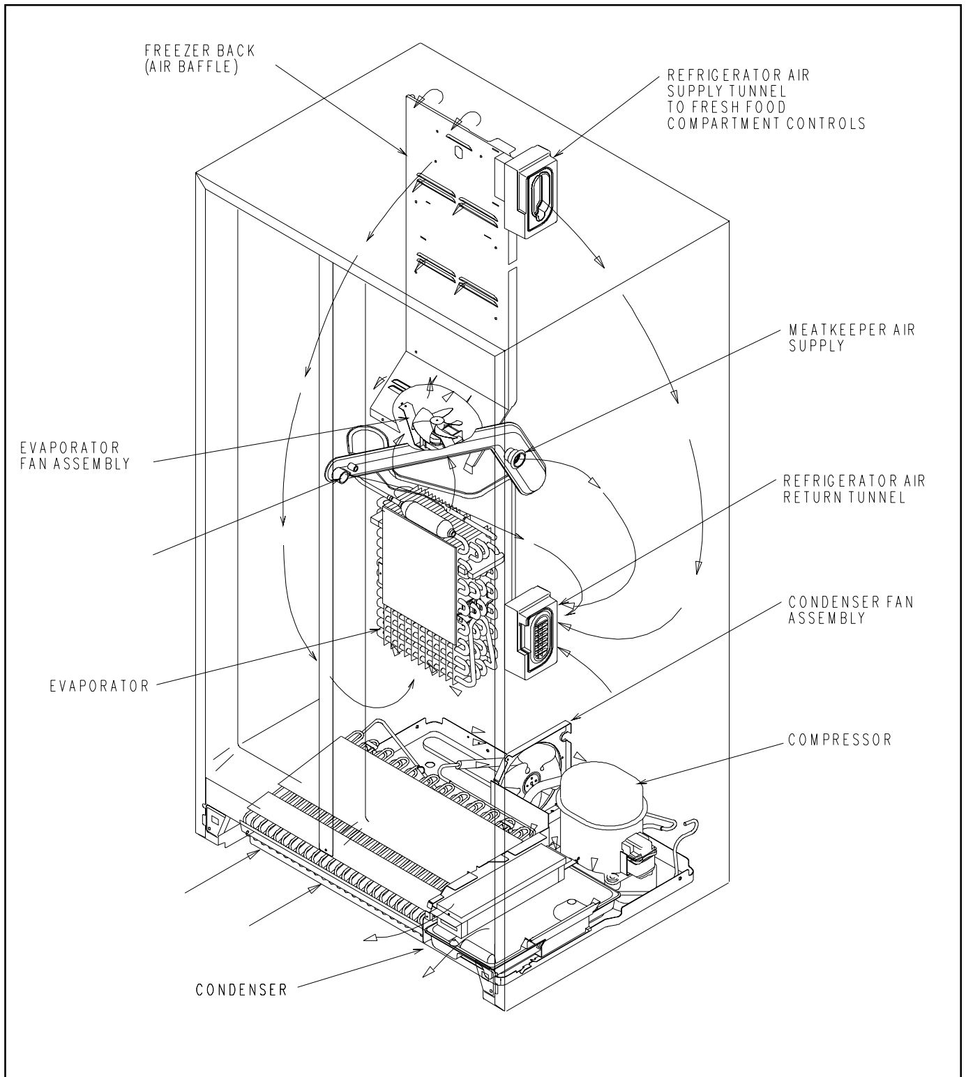
"T" Model Side x Side Air Flow Diagram 20 Cubic Foot Only
