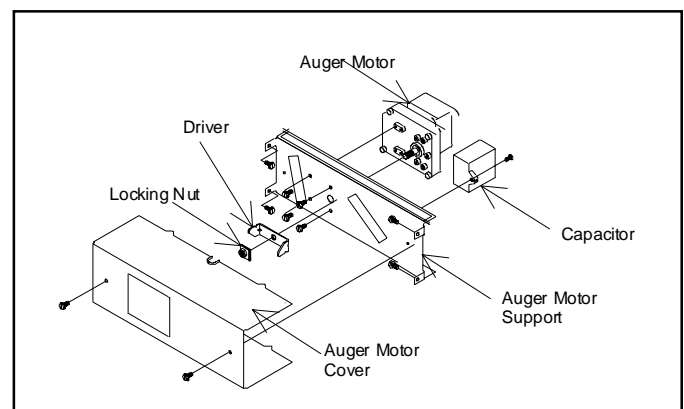
Auger Motor
