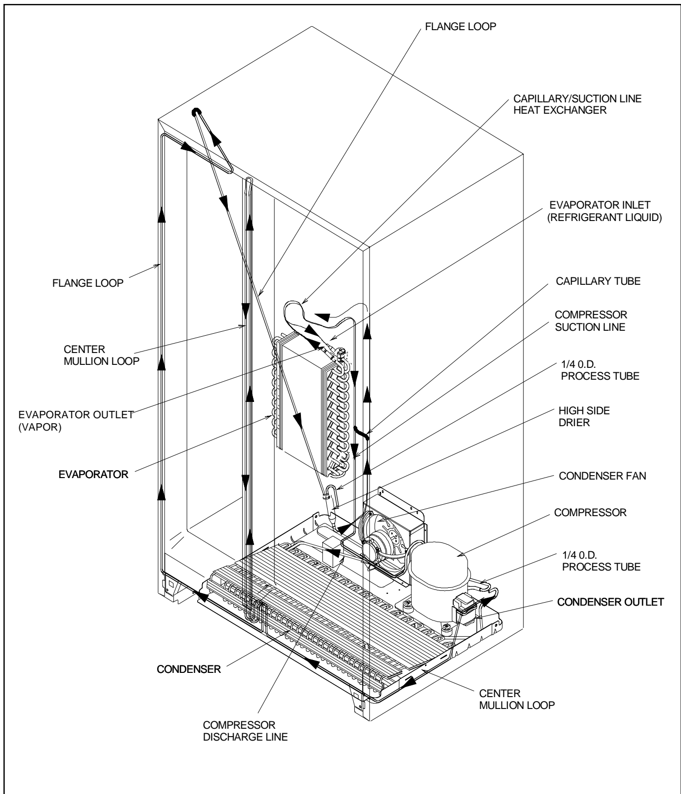
“T” Model Side x Side Refrigerant Flow Diagram 22/25/27 Cubic Foot Only
