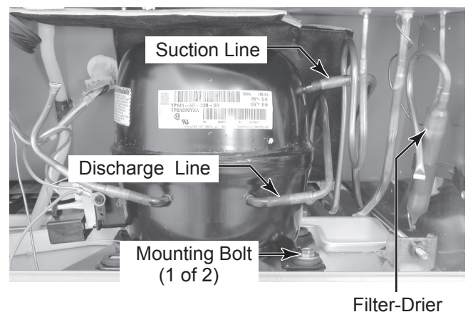
Compressor Filter-Drier
