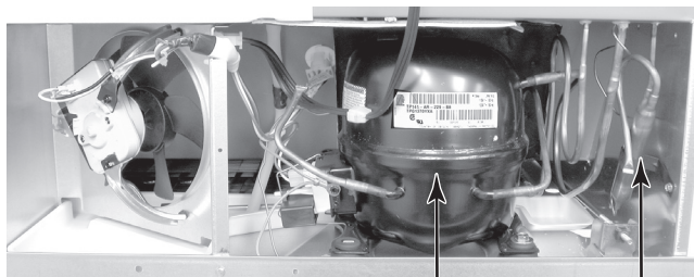
Compressor Filter-Drier
