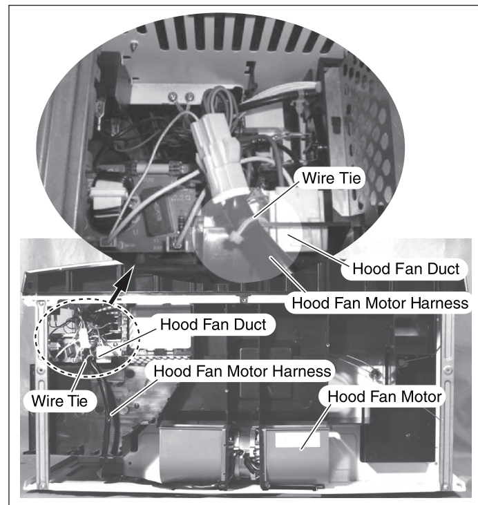
Figure 4-3. Hood Fan Motor Components
