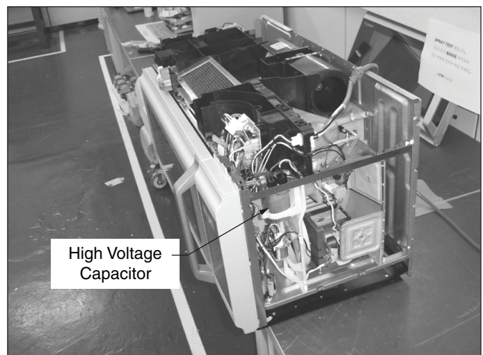
Figure 1-3. Capacitor Discharging NOTE: The illustration above gives a generalized location of the high voltage capacitor. Refer to the exploded view of the oven and cabinet for exact location.
