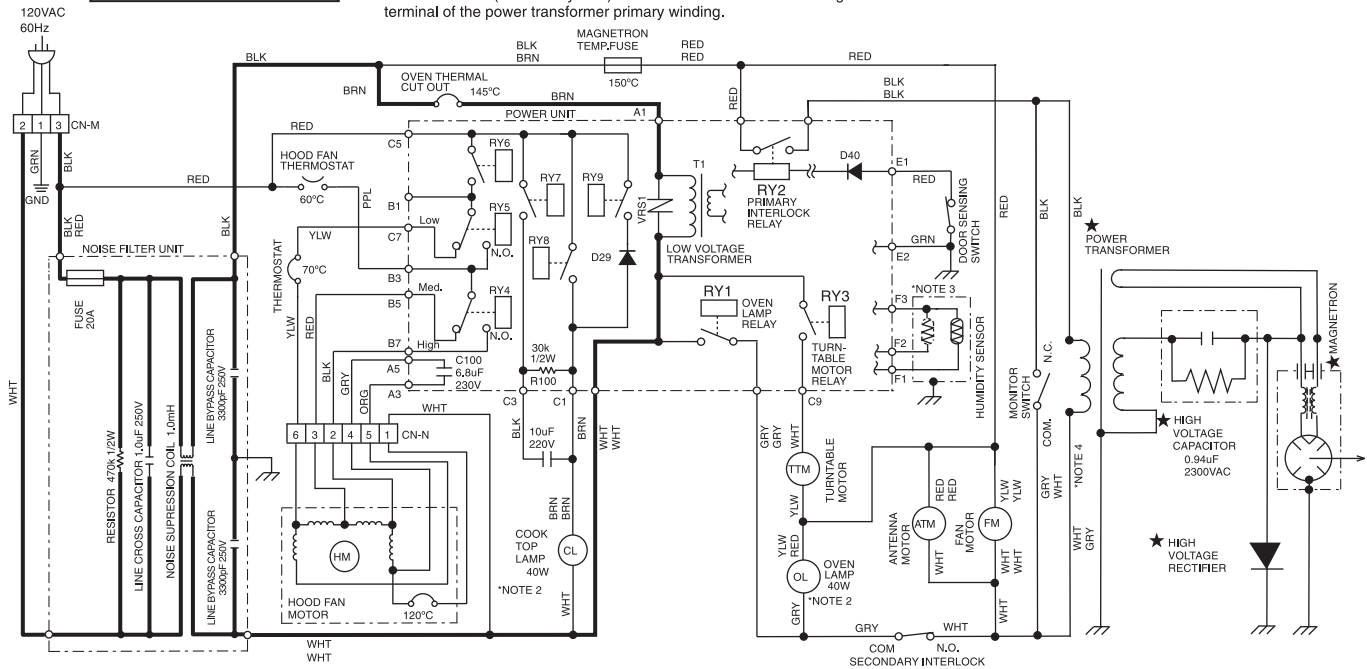
Figure 2-1. Microwave Oven Off Condition
