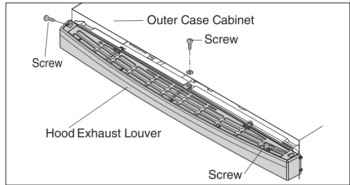
Figure 4-1. Outer Case Removal
