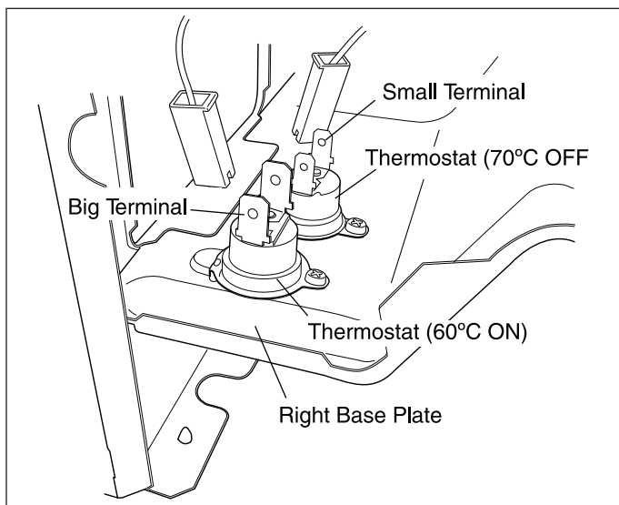
Figure 4-4. Thermostat Removal
