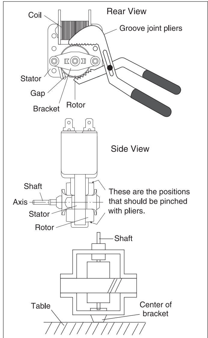
Figure 4-5. Fan Assembly Removal
