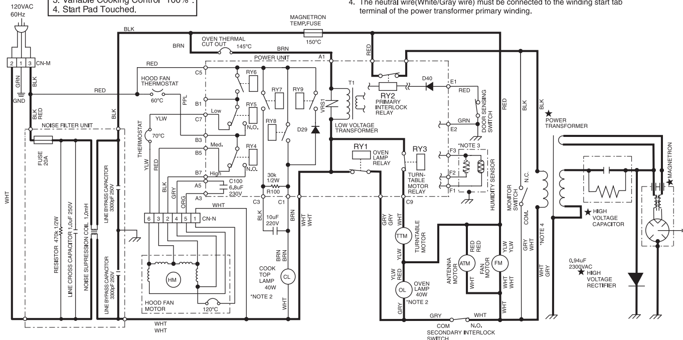
Figure 2-2. Oven Schematic-Microwave Oven Cooking Condition
