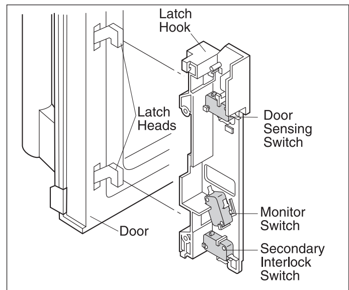
Figure 4-7. Latch Switch Adjustments
