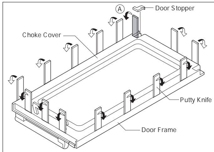
Figure 4-9. Door Disassembly
