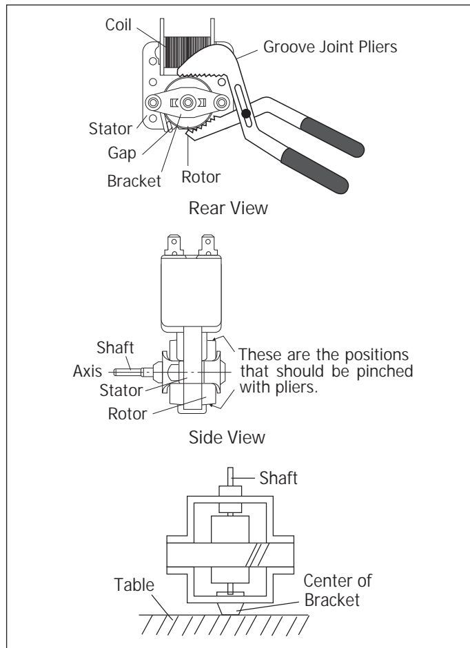
Figure 4-4. Door Switch Components
