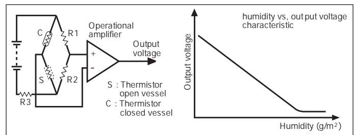
Figure 2-5. Humidity Sensor Operation
