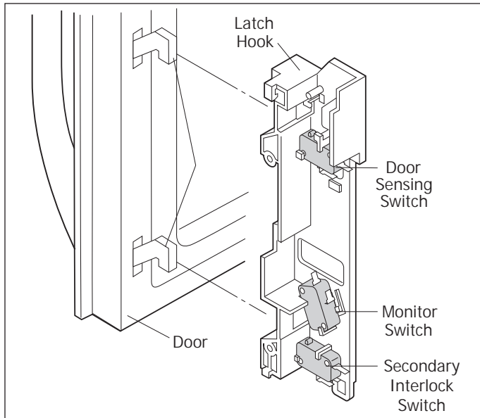
Figure 2-3. Door Open Mechanism
