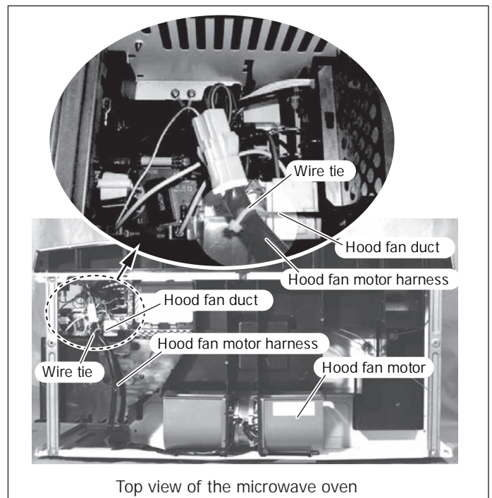
Figure 4-2. Top View Of The Microwave Oven
