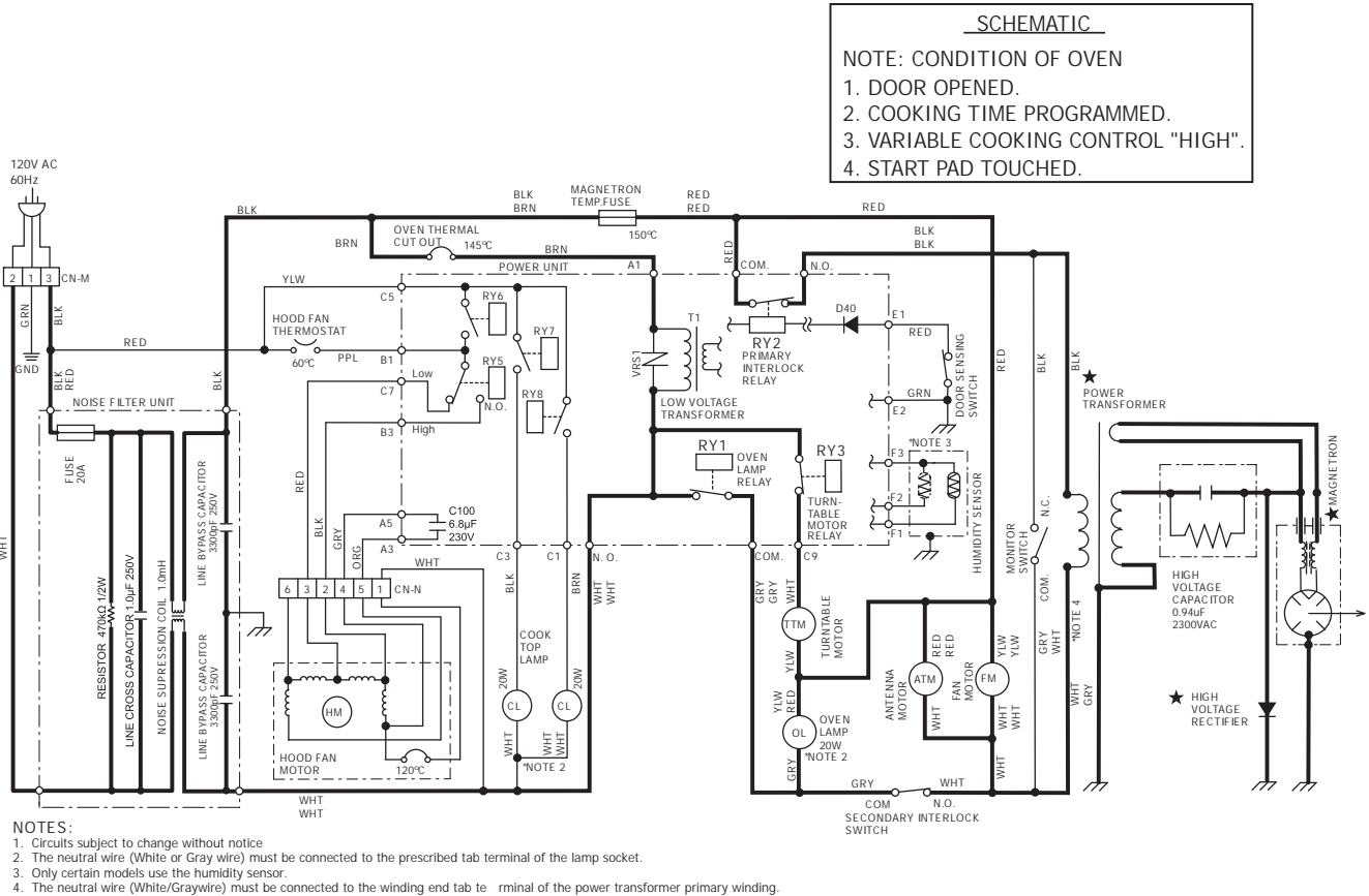
Figure 2-2. Oven ON (Cooking) Condition
