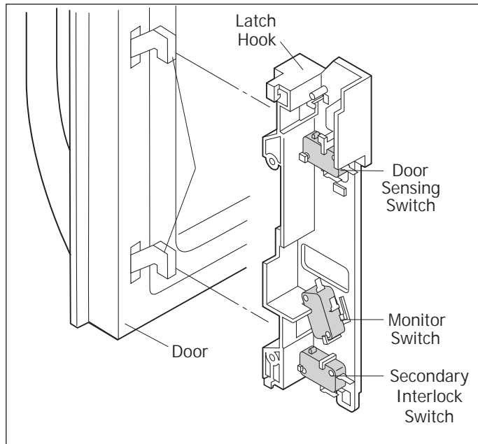
Figure 4-7. Door Disassembly
