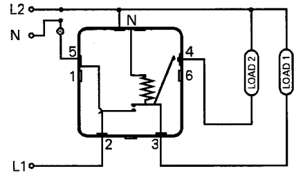
Wiring Diagram
