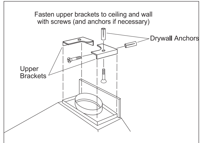
Figure 2-13 Upper Flue Bracket Installation
