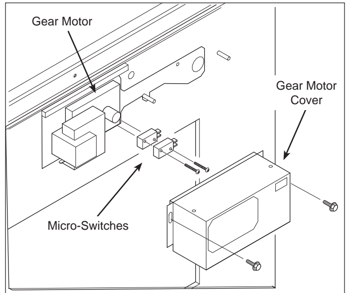
Figure 4-30 Micro-Switch Removal
