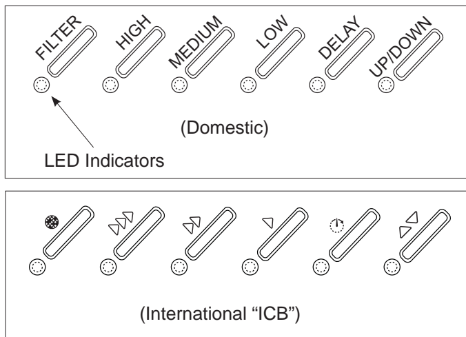
Figure 3-2 Downdraft Controls
