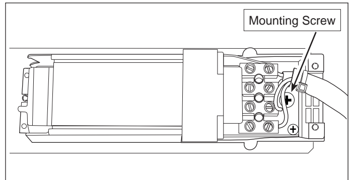
Figure 4-10 Disconnect Wire Harness
