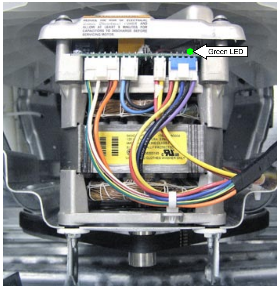
Inverter/Motor
