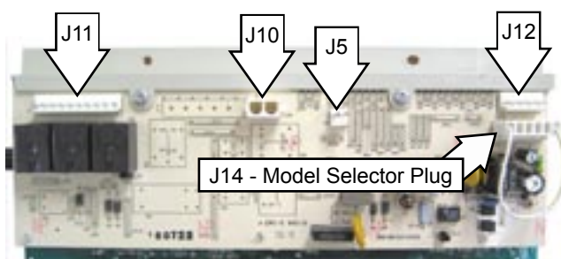
Main Control Board - Rear View
