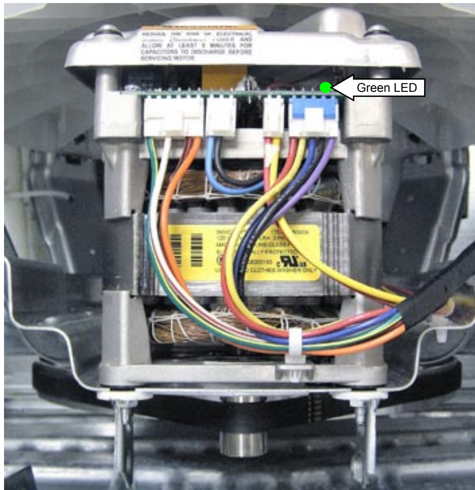
Inverter/Motor
