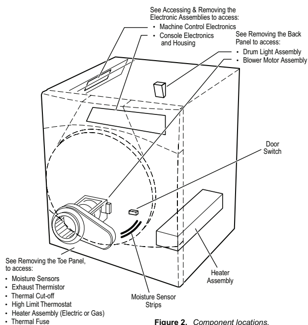
Figure 2. Component locations.
