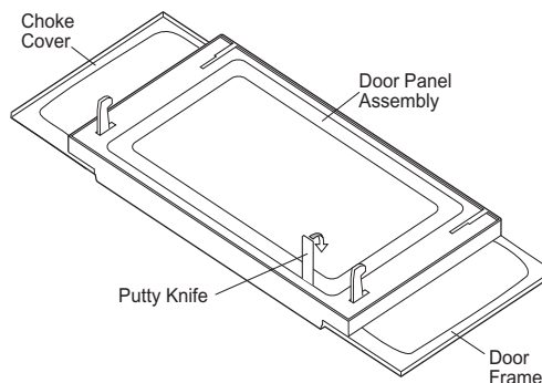
Figure C-5. Door Disassembly
