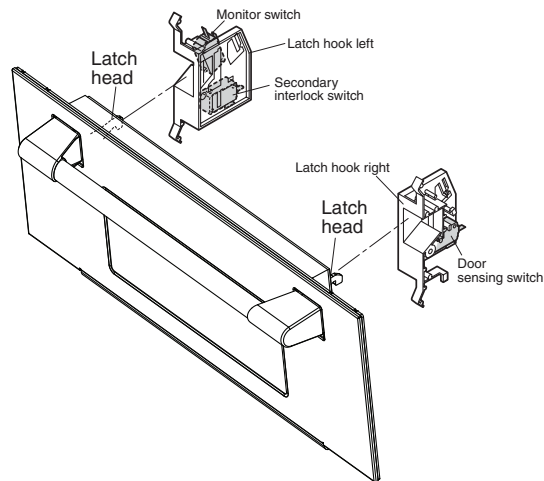
Figure C-2. Switches
