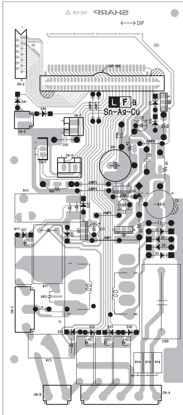
Figure S-4. Printed Wiring Board
