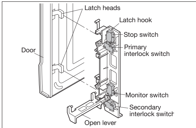
Figure D-1. Door Open Mechanism
