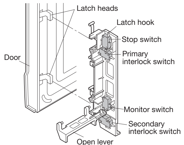
Figure C-1. Latch Switch Adjustments
