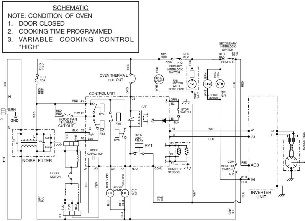
Figure O-1. Oven Schematic-Off Condition
