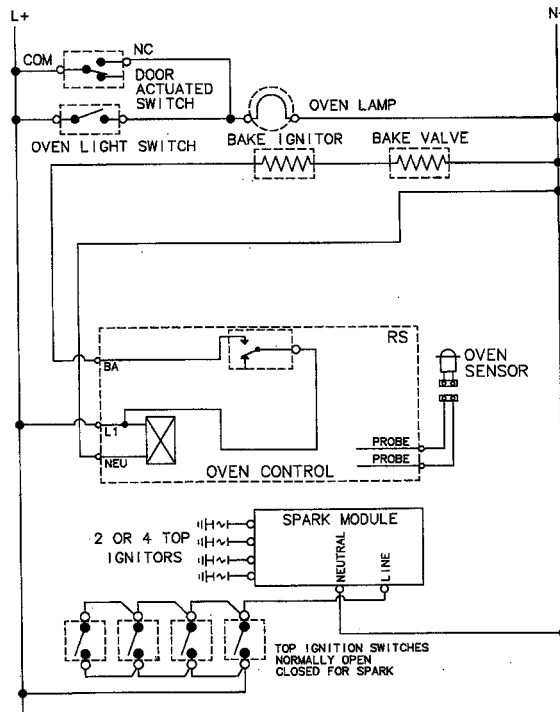
SCHMATIC
