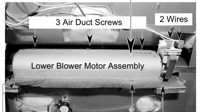
4 Mounting Screws
