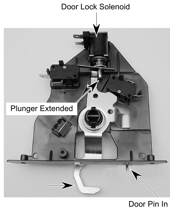
Door Closed & Locked
