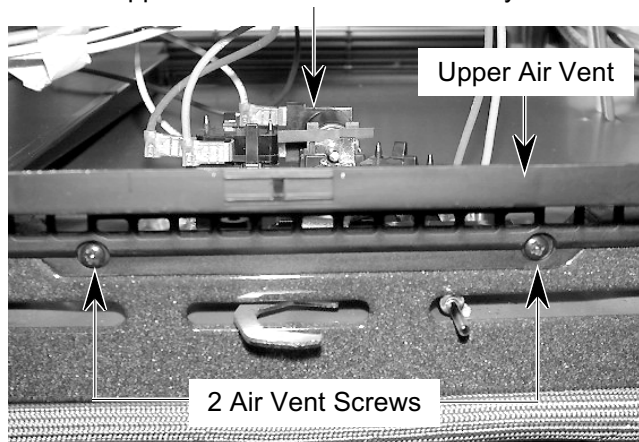
Upper Oven Door Latch Assembly
