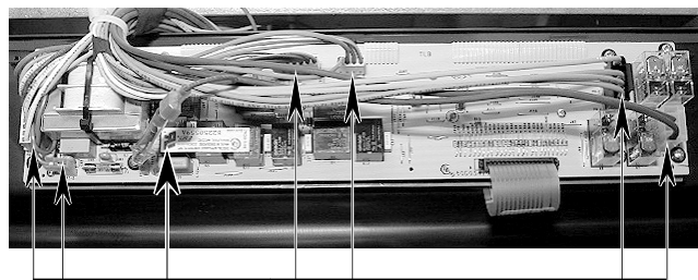
6 Wire Connectors
