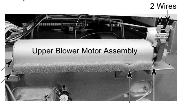
4 Mounting Screws
