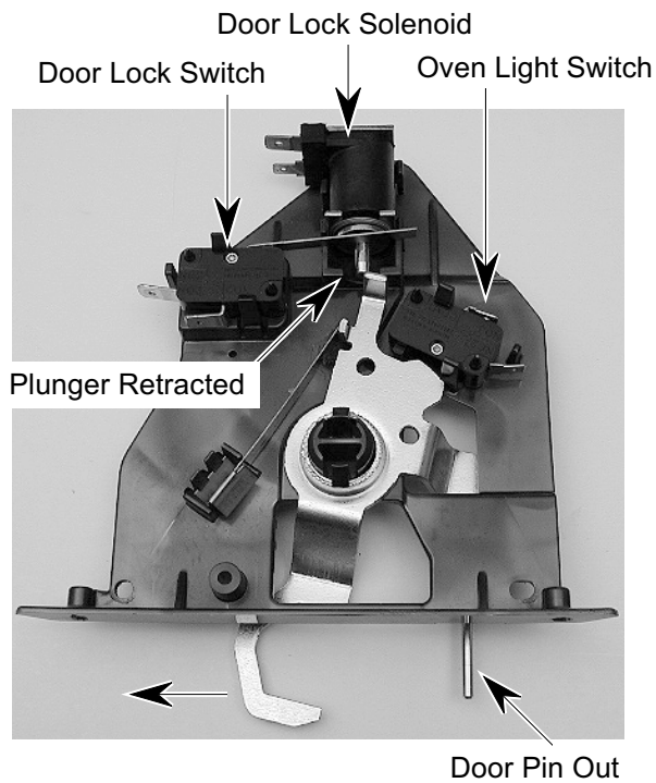
Door Open & Unlocked
