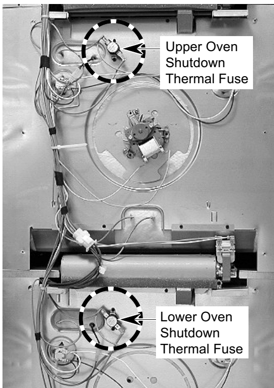
BACK OF OVEN
