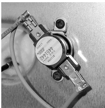
Oven Shutdown Thermal Fuse
