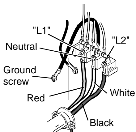
3-wire Cord Installed
