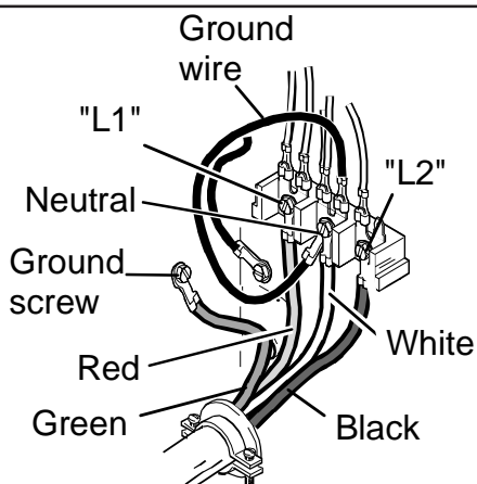
4-wire Cord Installed
